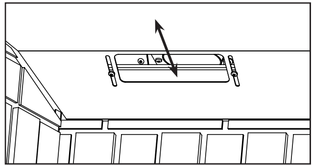
Figure 19: Baffle plate adjustment
