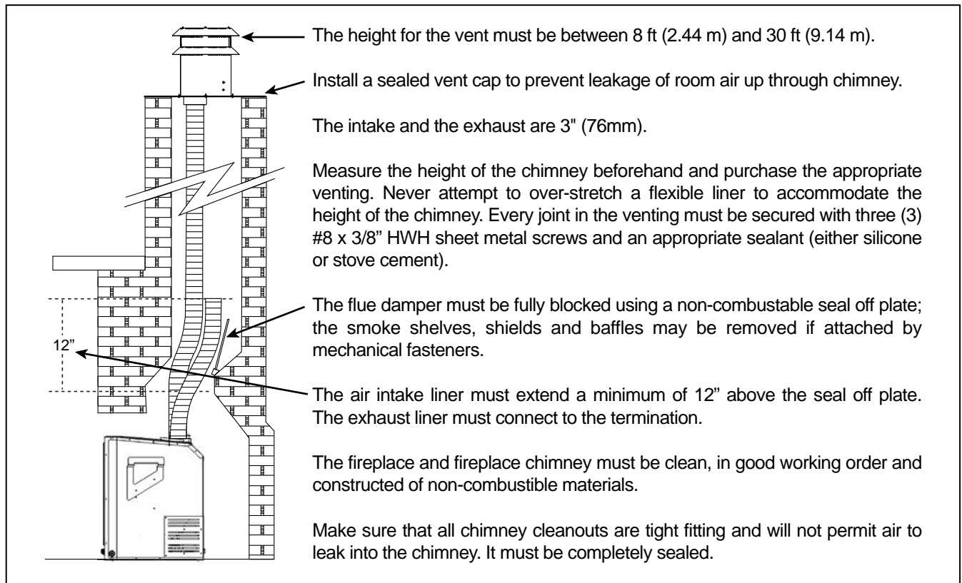
Figure 17: Alternate Installation of E33
