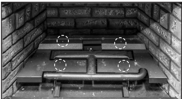
Figure 37: The log grate is removed next by simply lifting it off the grate tabs.
